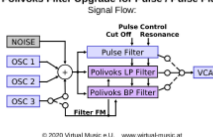
Polivoks Filter Upgrade for Pulse / Pulse Plus
